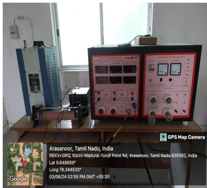
WIND – SOLAR HYBRID SYSTEM IN RENEWABLE ENERGY SOURCES LABORATORY
